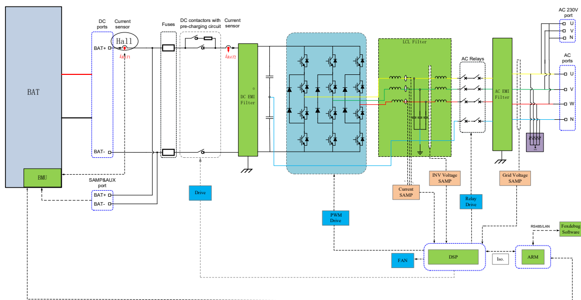
Figure 1: Schematic overview circuit diagram
