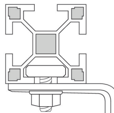
Dachhaken
